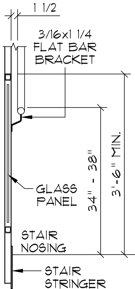
END VIEW
