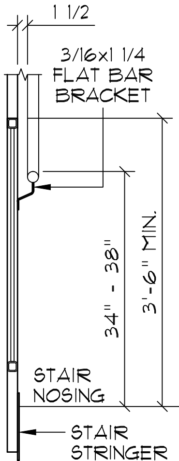
END VIEW
