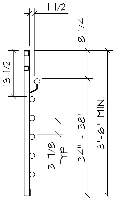
END VIEW
