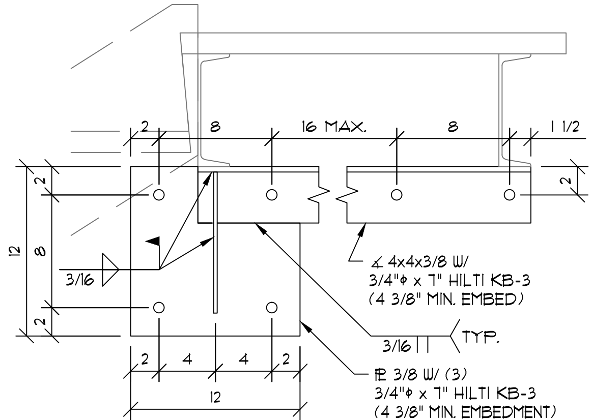
SECTION A
