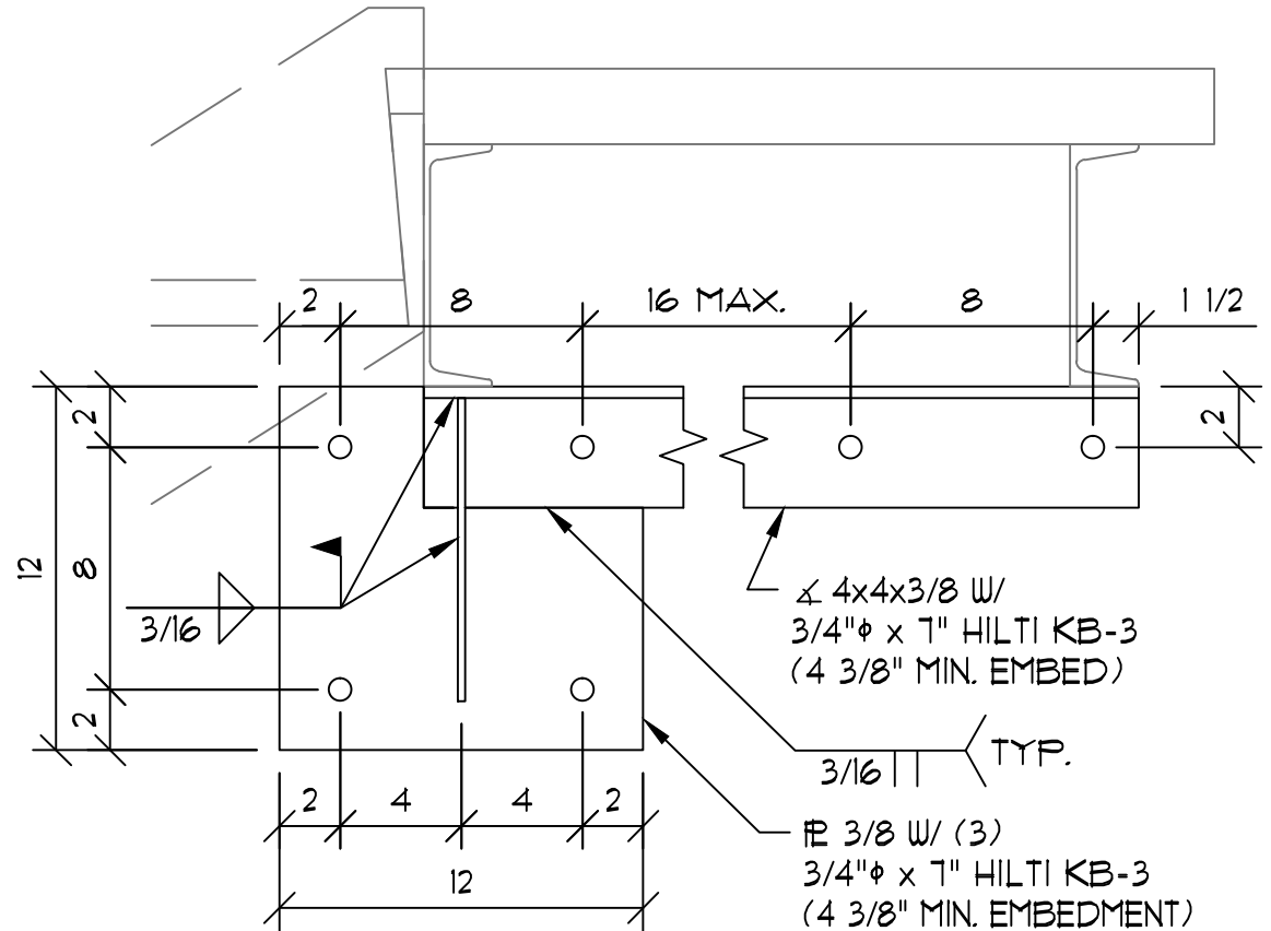
SECTION A
