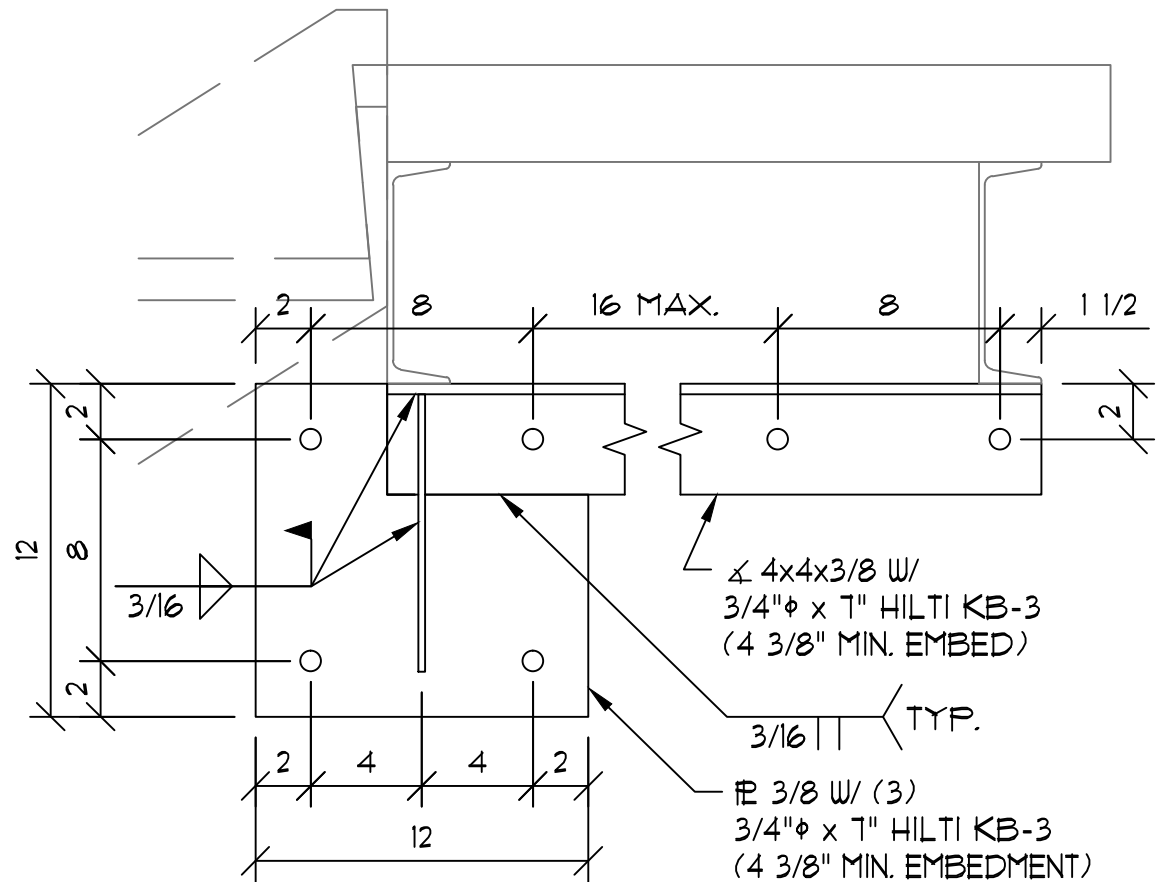
SECTION A
